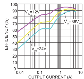
Efficiency vs. Load Current V_{OUT} = 3.3V
