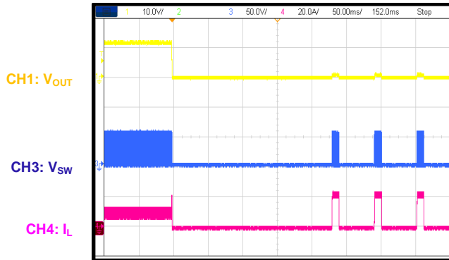
Short-Circuit Protection Entry I_{OUT} = 10A to short circuit
