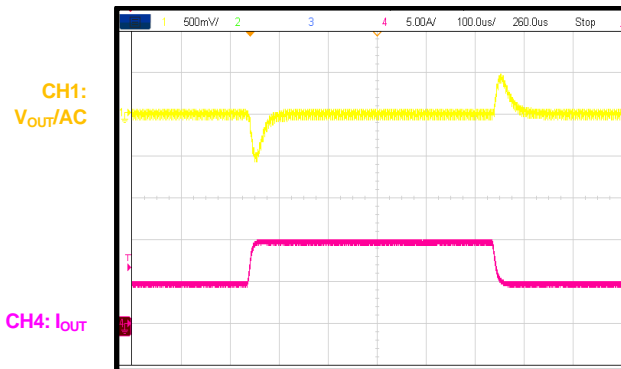
Load Transient I_{OUT} = 5A to 10A , 500mA/\mu s
