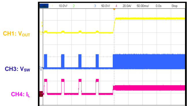
Short-Circuit Protection Recovery Short circuit to I_{OUT} = 10A
