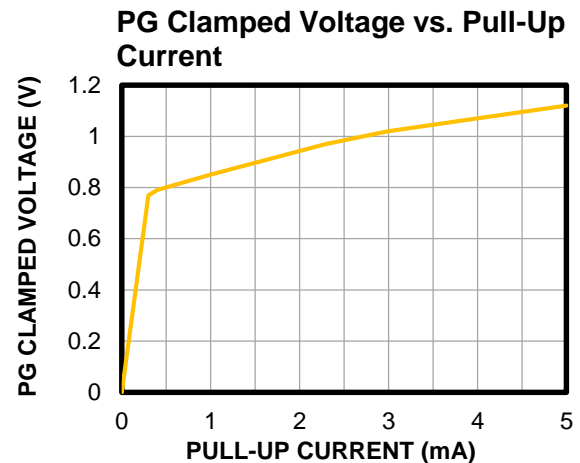
Figure 3: PG Clamped Voltage vs. Pull-Up Current
