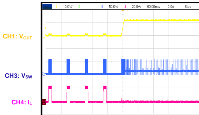
Short-Circuit Protection Recovery Short circuit to I_{OUT} = 0A
