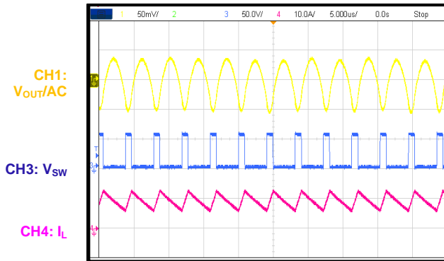
Steady State I_{OUT} = 10A
