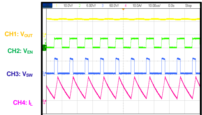
SYNC Function f_{SYNC} = 100kHz , I_{OUT} = 10A
