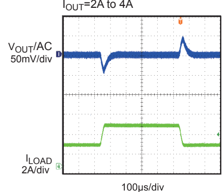
Load Transient Response I_{OUT}=2A to 4A
