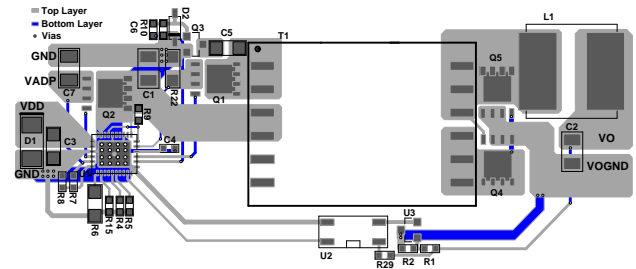
Figure 17: Recommended PCB Layout for Forward Topology
