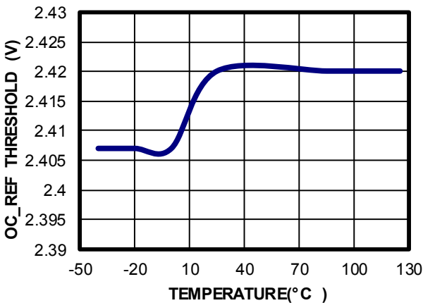
O CREF Threshold vs. Temperature O CREF = 2.4V
