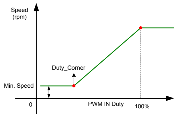
Figure 3: Programmable Speed Curve
