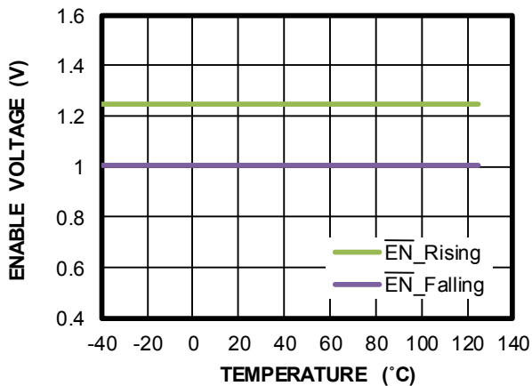
\overline{\text{EN}} Rising/Falling Threshold vs. Temperature T_A = -40^\circ\text{C} to +125^\circ\text{C}
