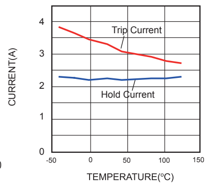
Trip and Hold Current vs. Temperature
