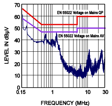
EMI V IN = 120V AC V OUT = 27V
