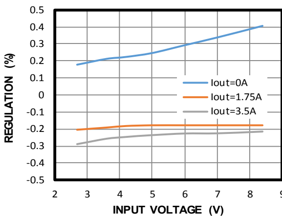
Line Regulation PSM
