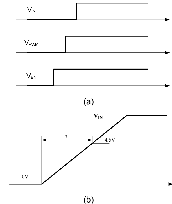
Figure 3: Input Voltage Rise-Time Indicator for a 6-String LED Application
