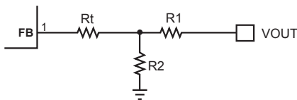
Figure 6— T-type Network
