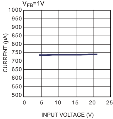
Enable Supply Current vs. Input Voltage
