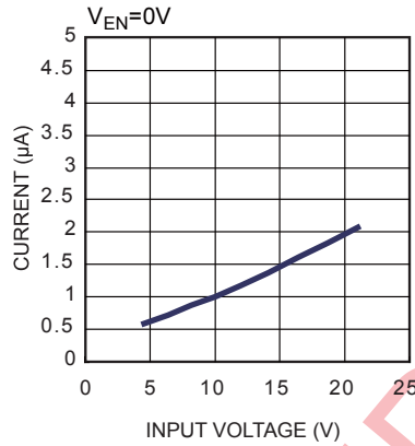
Disabled Supply Current vs. Input Voltage
