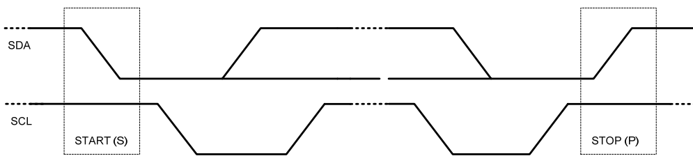
Figure 8: START and STOP Conditions
