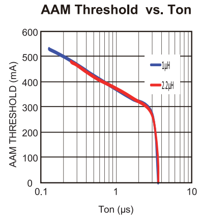
Figure 9: AAM Threshold decreases with Ton Increases.
