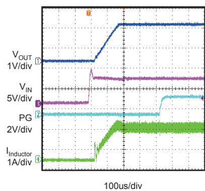
Power up
