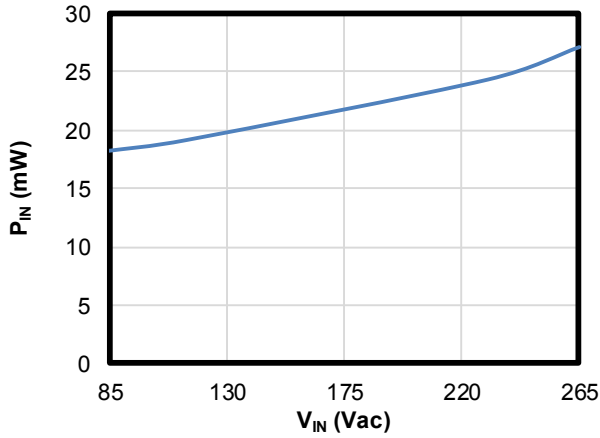
No-Load Consumption
