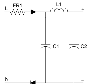
Figure 9: Half-Wave Rectifier
