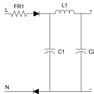
Figure 8: Half-Wave Rectifier
