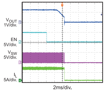
Shutdown Through EN I_{OUT} = 6A
