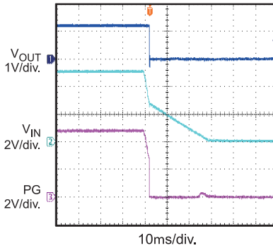
Power Good Through Shutdown I_{OUT} = 6A
