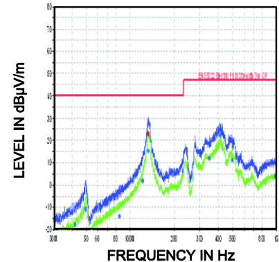
Radiation EMI Performance
