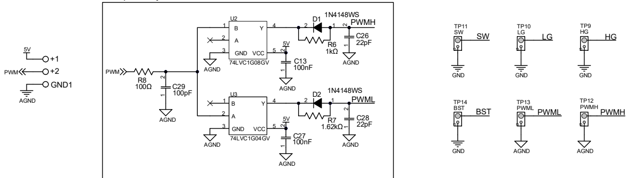
Figure 2: Evaluation Board Schematic
