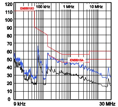
Conduction EMI
