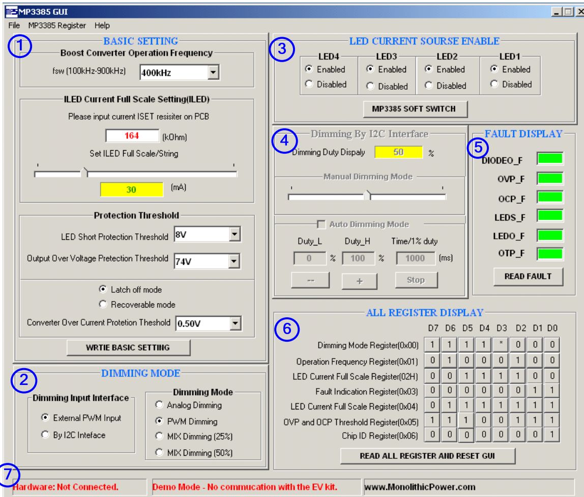
Figure 2 — MP3385 GUI
