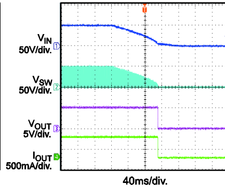
Power Ramp Down V_{IN}=50V
