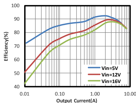
Efficiency vs. Output Current V OUT =1V, L=1μH (DCR=4.6mΩ)
