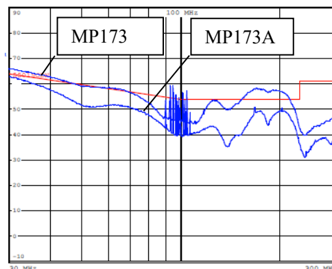
RE Performance
