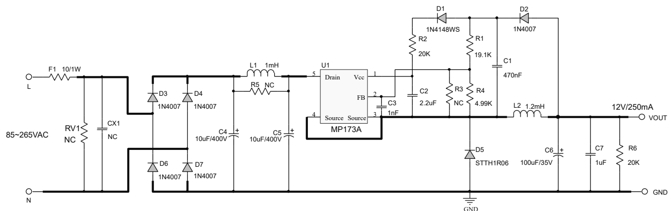
Figure 1: Schematic
