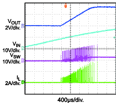
Start Up Through VIN V_{IN} = 22V , I_{OUT} = 0A
