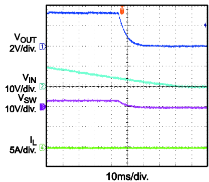
Shut Down Through VIN V_{IN} = 22V , I_{OUT} = 0A
