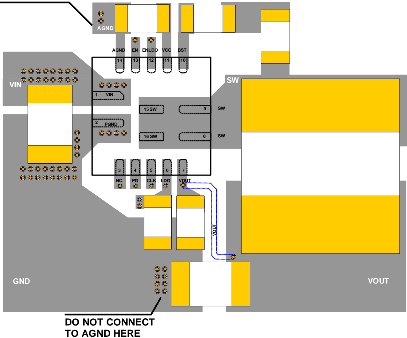
Figure 9—Recommend Layout
