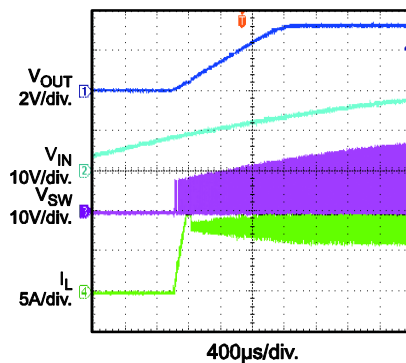
Start Up Through VIN V_{IN} = 22V , I_{OUT} = 8A
