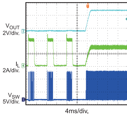
SCP Recovery Short Circuit to I_{OUT}=3A
