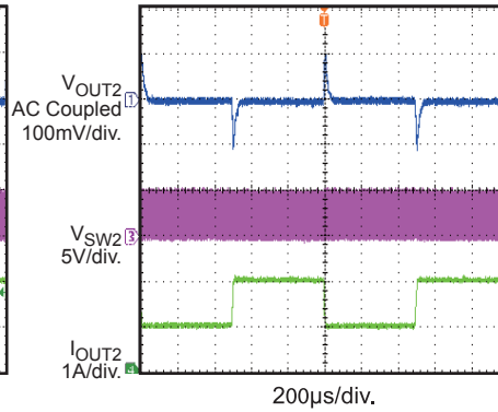
Load Transient 1A Transient to 2A, 2.5A/ \mu S speed
