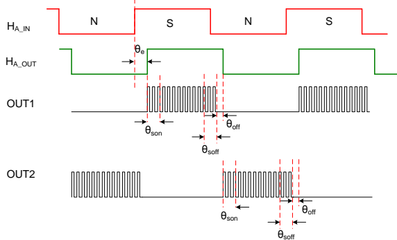
Figure 2: Timing Diagram
