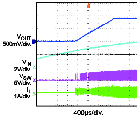
V IN Power Up without Load I_{OUT} = 0A
