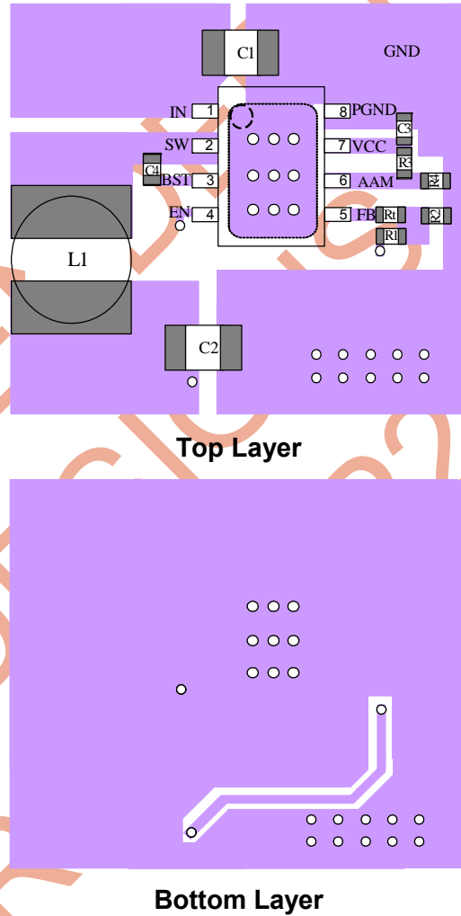
Figure 7—PCB Layout
