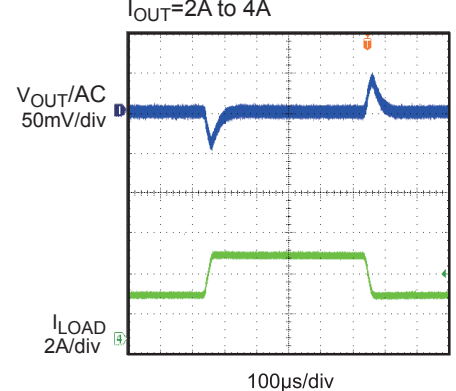
Load Transient Response I_{OUT}=2A to 4A
