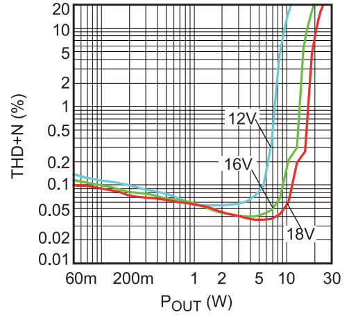
THD+N vs. P OUT (1kHz, 8Ω+66μH)
