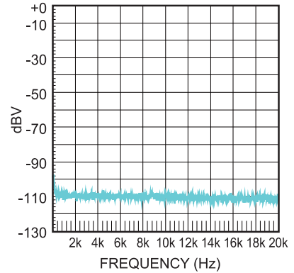
FFT Noise Floor Test (18V, 8Ω+66μH)
