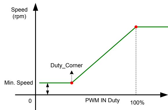
Figure 3: Programmable Speed Curve
