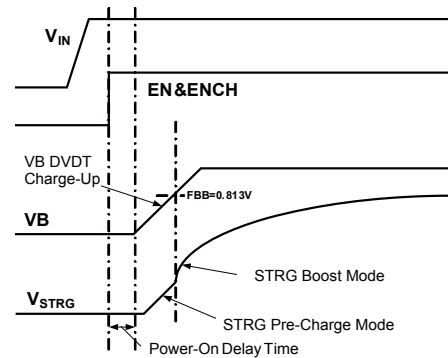
Figure 1: Charging Process
