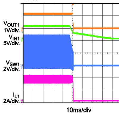
VIN Power-Down with 3.5A Load (CH1)
