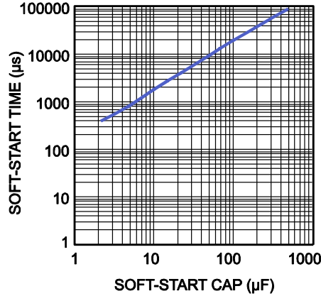
Soft-Start vs.Cap
