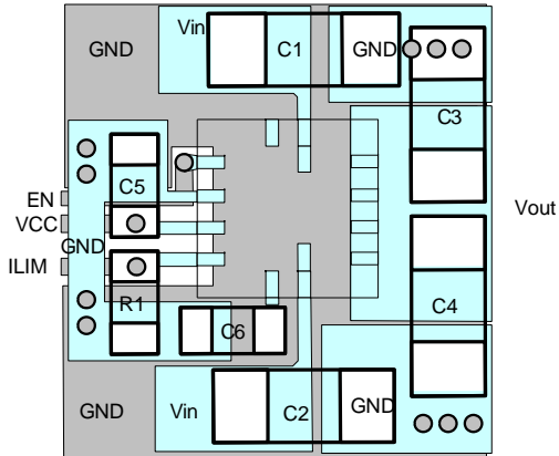
Figure 5: Recommended Layout
