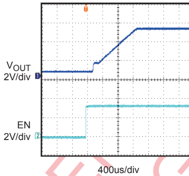
Turn on Delay and Rise Time with 1uF Load, no Cdv/dt
