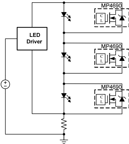
Figure 1. LED Open Protection Circuit
