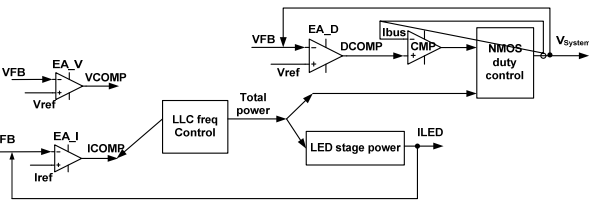
Figure 4B: MP4655 Control Scheme at PWM Dimming On
