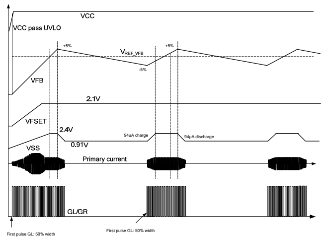
Figure 3: LLC Soft-Burst Operation at Standby Mode
