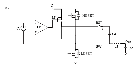
3b: BST Charging Path when HS-FET and LS-FET are Both Off
