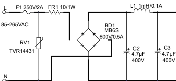
Figure 9: 2kV Surge Solution
