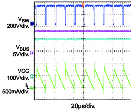
Steady State@220VAC
