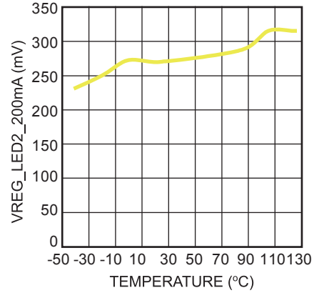
V_LED2(20mA) vs. Temperature Chart
