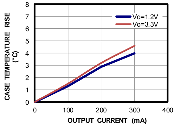
T RISE vs. Output Current
