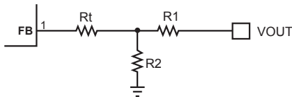
Figure 6— T-type Network
