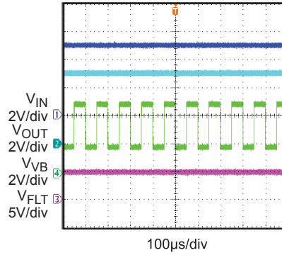
Battery OVP within Blanking Time (No Load)
