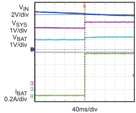
Input OVP Recovery V_{IN} from 6V to 5V, MODE=1, R_{CHG}=3.6k , W/ Battery
